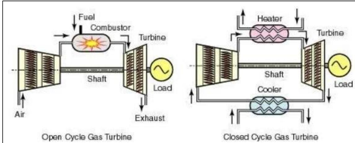
Typical Open and Close cycle Gas Turbine
