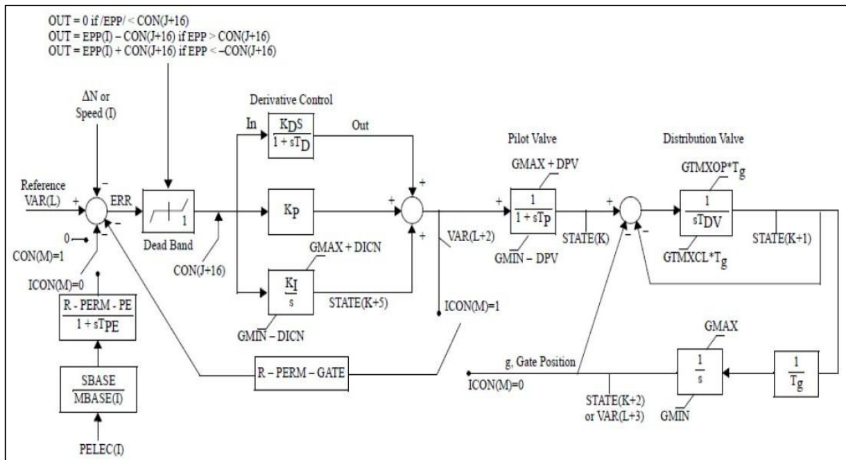
Governor and Hydraulic Actuators
