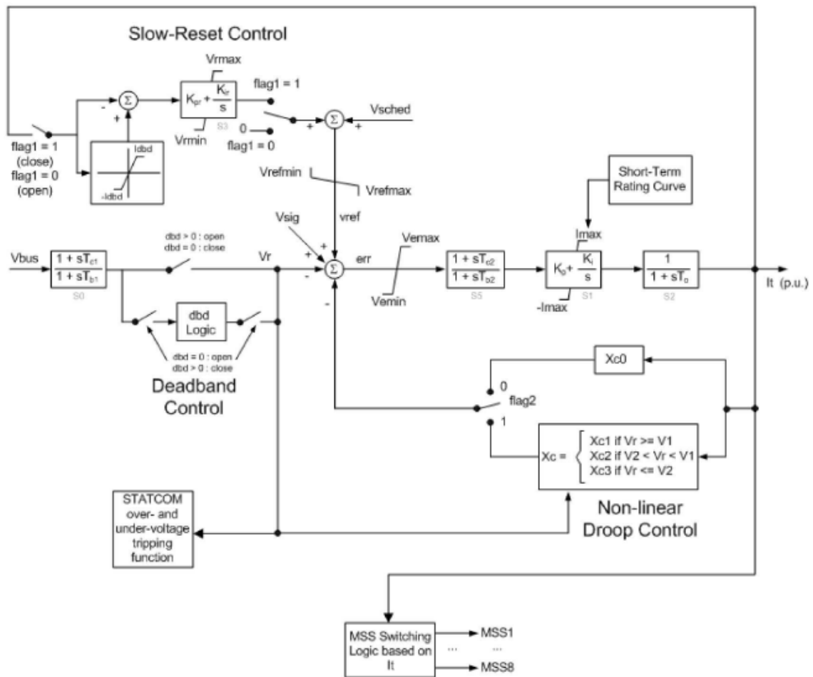
Illustration of STATCOM characteristic for model SVSMO3T2
