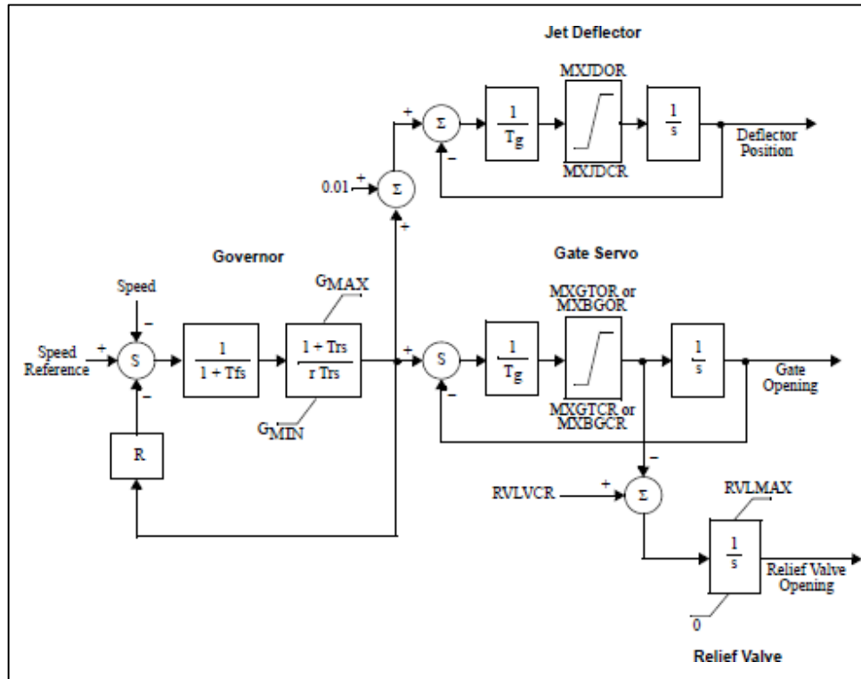
Governor and Hydraulic Actuators
